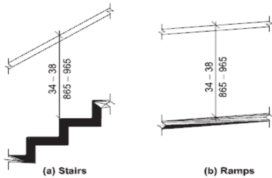
Fig. 505.4 Handrail Height
