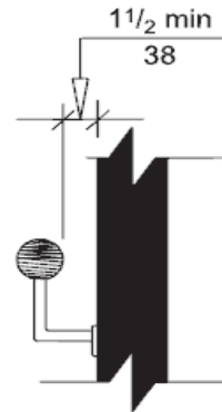
Fig. 505.5 Handrail Clearance
