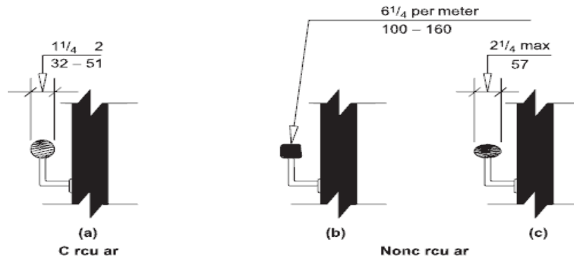
Fig. 505.7 Handrail Cross Section
